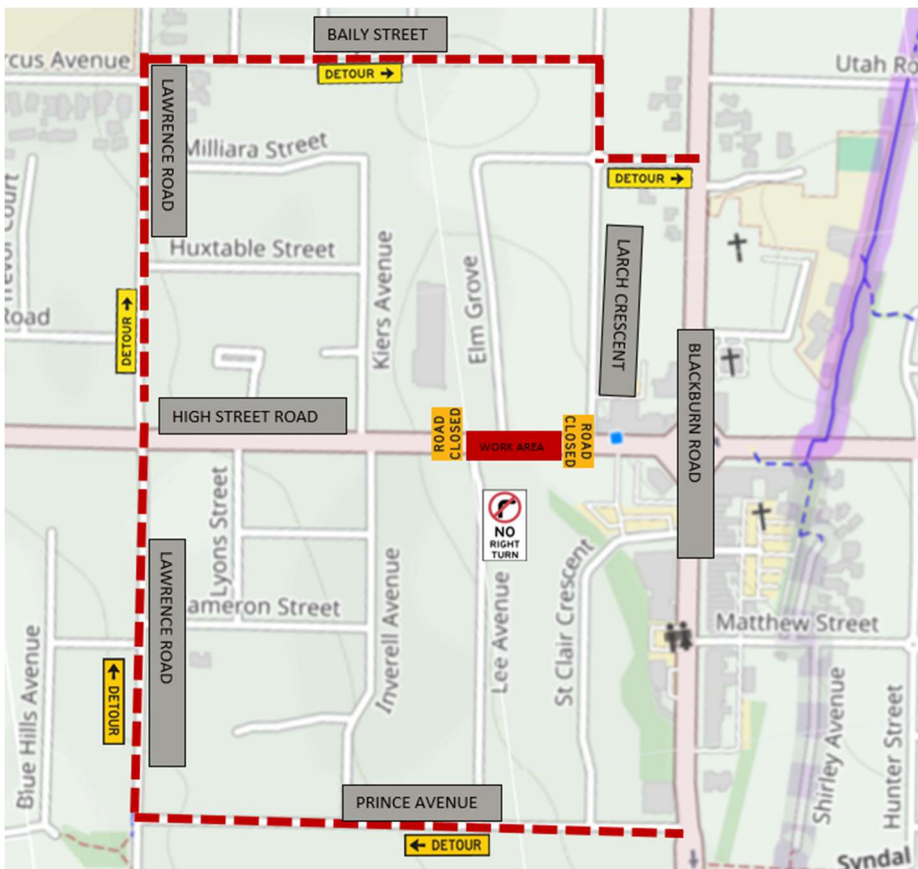
Figure 1: Work area and local traffic detour routes
